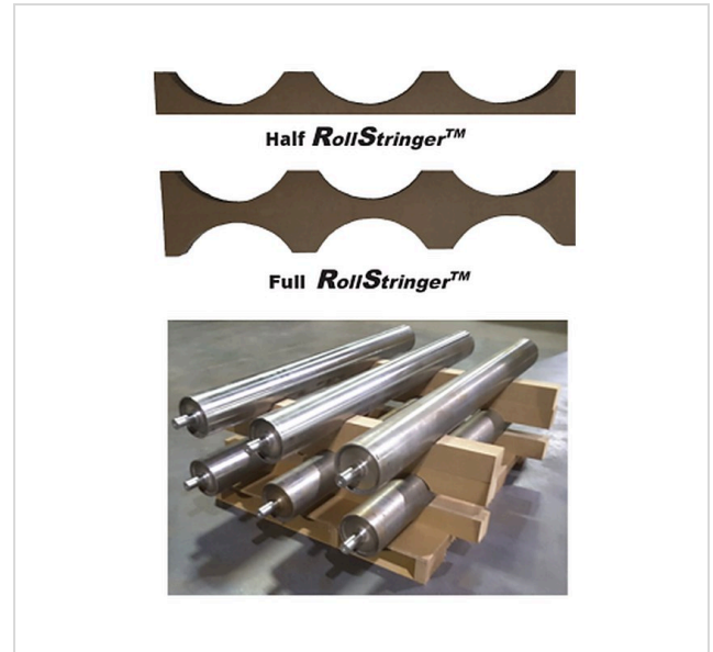
Half and Full RollStringer™ Support profiles, and RollStringer™ Supports holding steel rolls.
